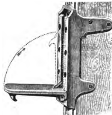
FIG. 50.—Adjustable Closing Step (Section 192).
